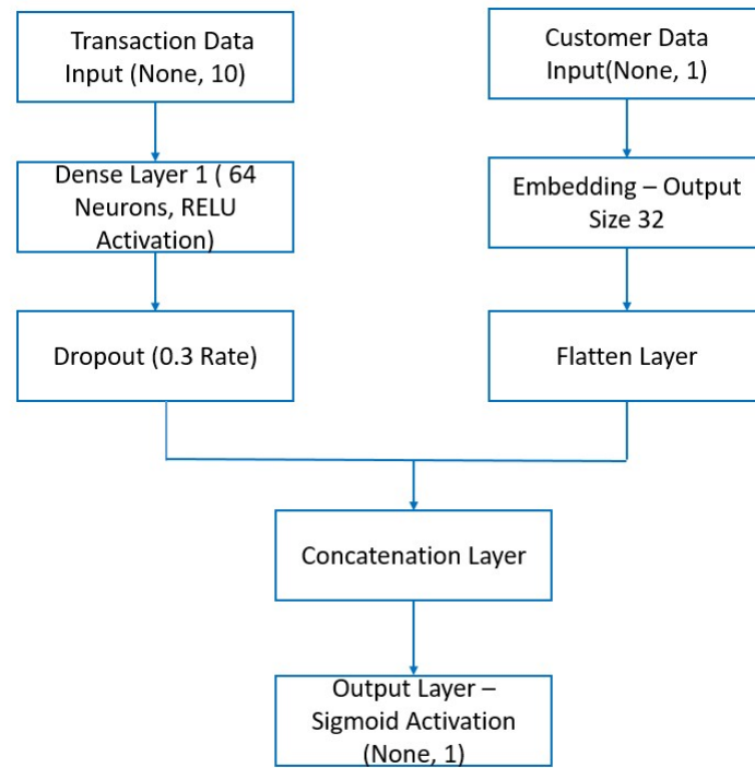
Figure 2. Model Architecture
