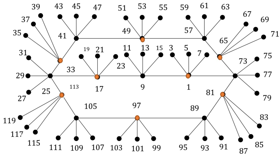
Figure 13. Super lehmer-3 mean labeling of (S(\theta_7)) \odot \bar{K}_3
