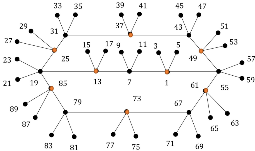
Figure 11. Super lehmer-3 mean labeling of (S(\theta_7)) \odot \bar{K}_2
