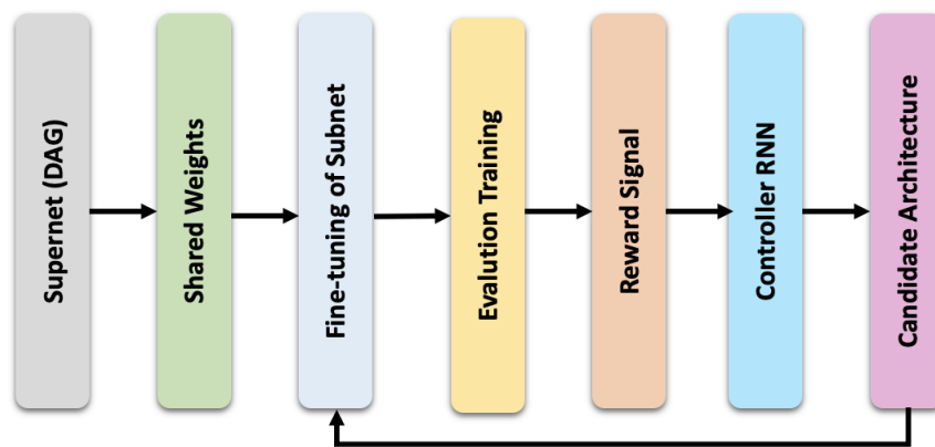
Figure 5. Architecture of Proposed ENAS
