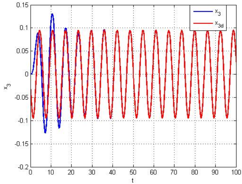
Figure 2. Output tracking x_3 to x_{3d} for the system relative degree 2
