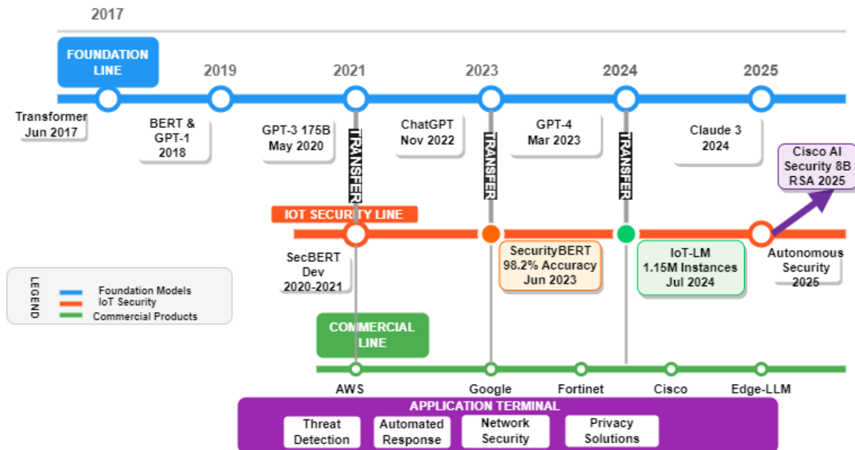
Figure 1. Timeline of LLM Evolution and IoT Security Applications: From BERT to IoT-Optimized Models
