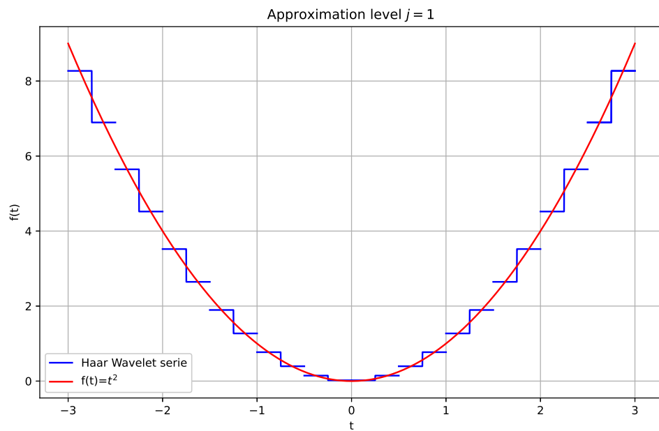
Figure 4. Haar Wavelet Series Representation with j = 1
