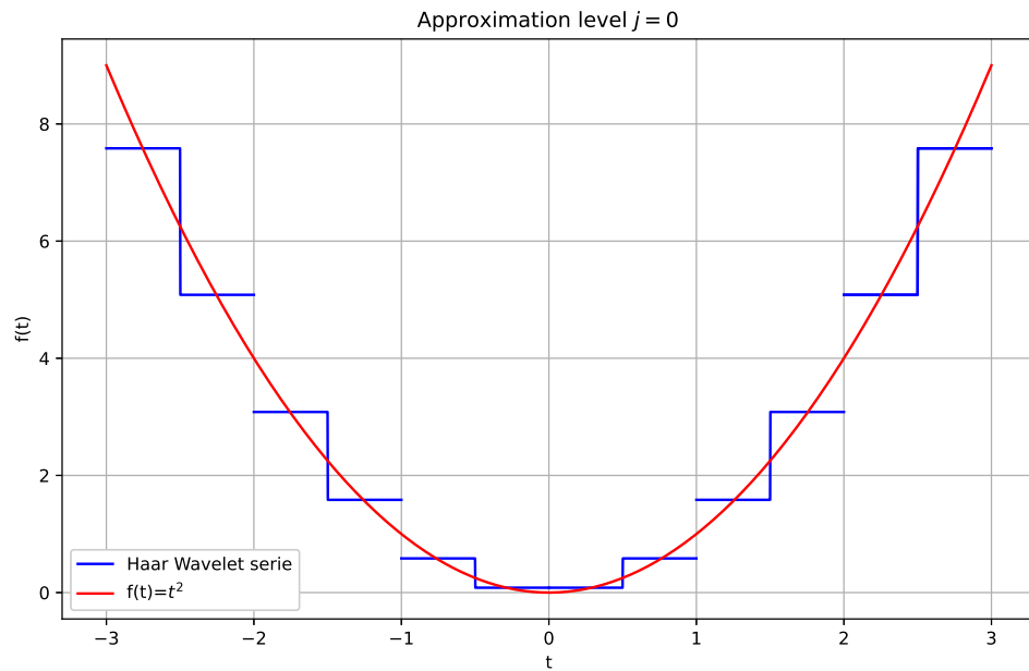
Figure 3. Haar Wavelet Series Representation with j = 0
