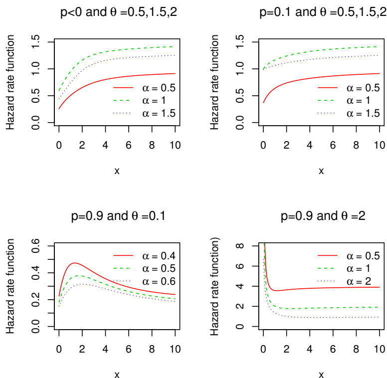
Figure 2. Plots of the hazard rate function for selected values of parameters
