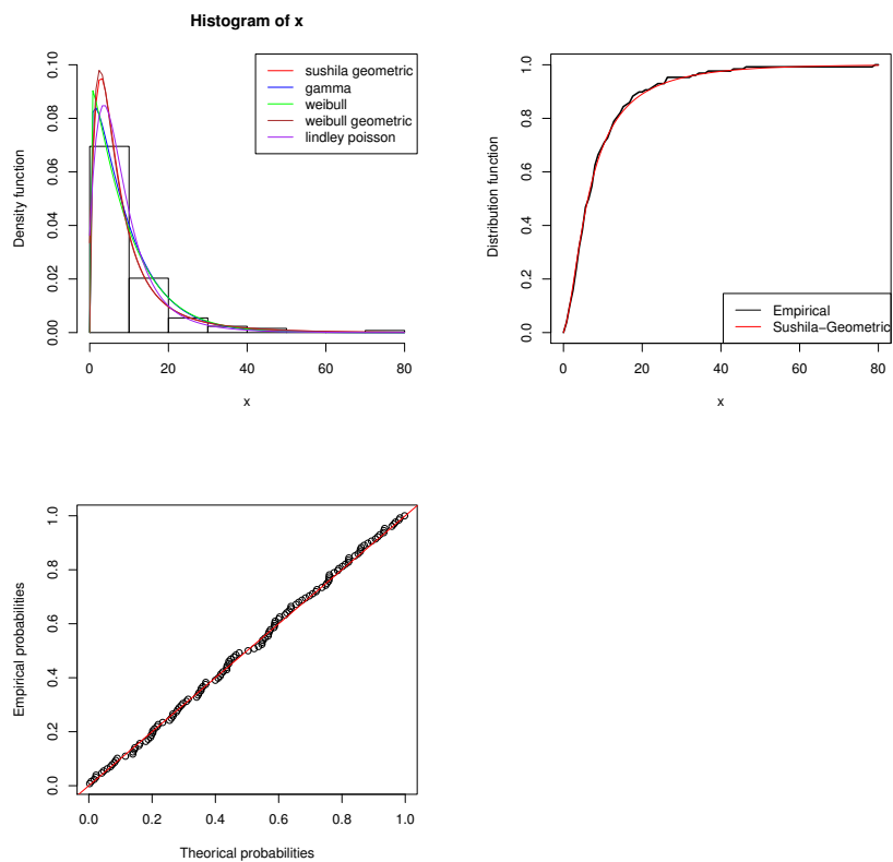
Figure 4. Plots of the estimated pdf and cdf and p-p plot of the SG model for data set 1
