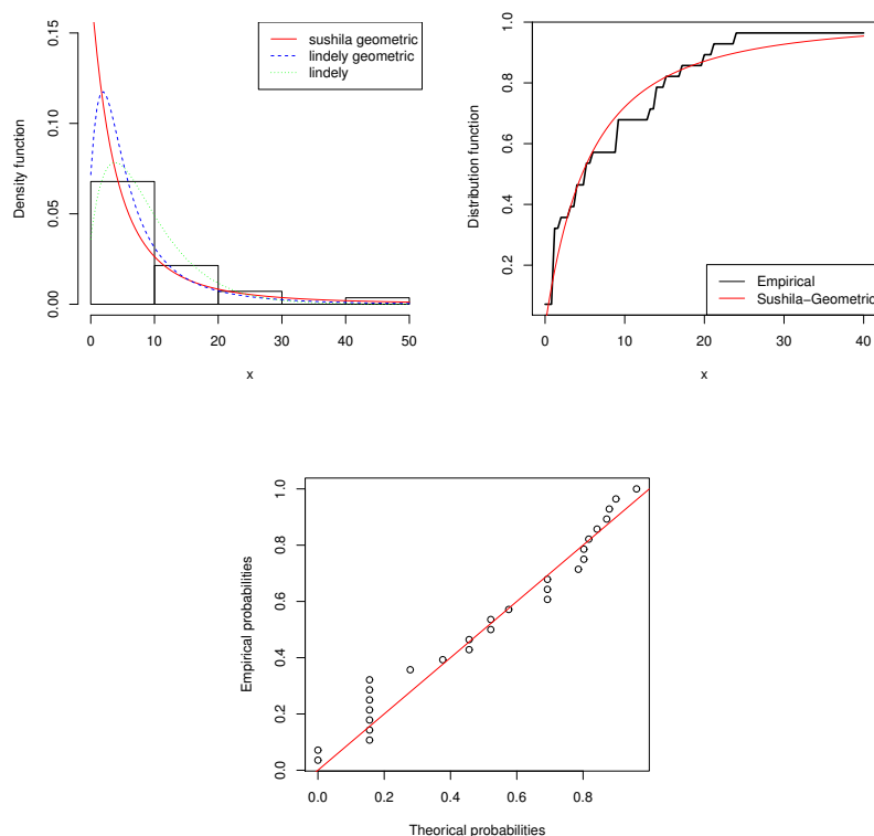
Figure 5. Plots of the estimated pdf and cdf and p-p plot of the SG model for data set2
