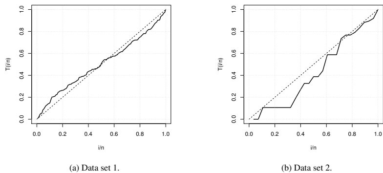
Figure 3. The empirical TTT plots of the two data sets.
