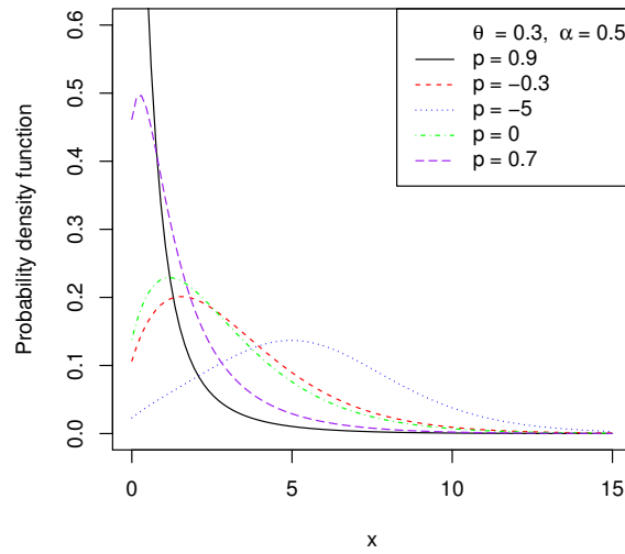
Figure 1. Plots of PDF of SG for selected values of parameters.
